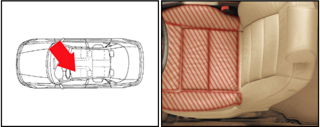
Z6 Driver's Seat Heating Element
