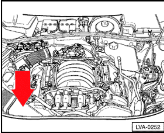
V101 Secondary Air Injection (AIR) pump motor (2.8 ltr. engine)
