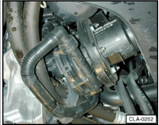
V101 Secondary Air Injection (AIR) pump motor (2.8 ltr. engine)
