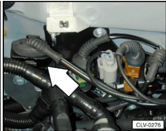
T4b Connector, 4-pin, black " (2.8 ltr. engine)
