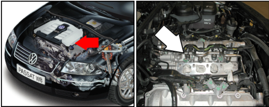
N86 Cylinder 8 Fuel Injector (4.0 ltr. engine)
