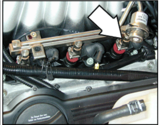
N84 Cylinder 6 Fuel Injector (2.8 ltr. engine)
