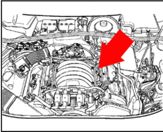
N84 Cylinder 6 Fuel Injector (2.8 ltr. engine)
