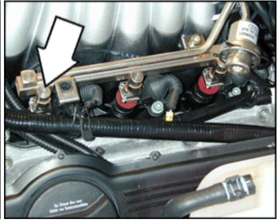
N33 Cylinder 4 Fuel Injector (2.8 ltr. engine)
