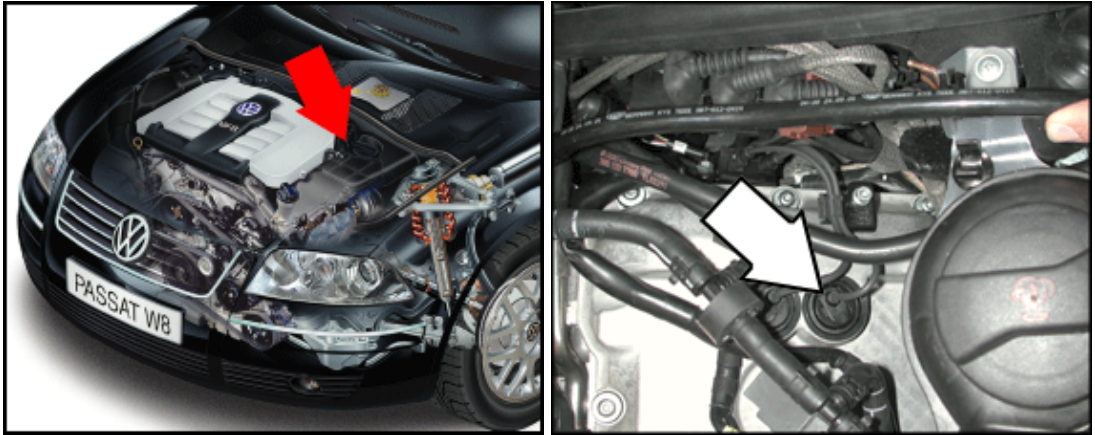
N319 Camshaft Adjustment Valve 2 (exhaust) (4.0 ltr. engine)
