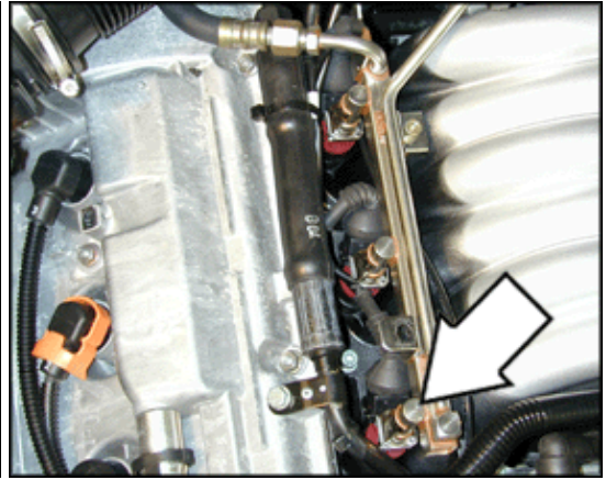
N30 Cylinder 1 Fuel Injector (2.8 ltr. engine)
