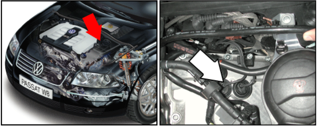
N208 Valve -2- for camshaft adjustment (4.0 ltr. engine)
