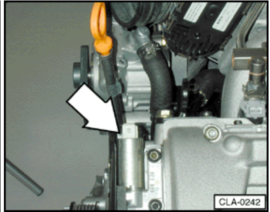
N208 Valve 2 for camshaft adjustment (2.8 ltr. engine)
