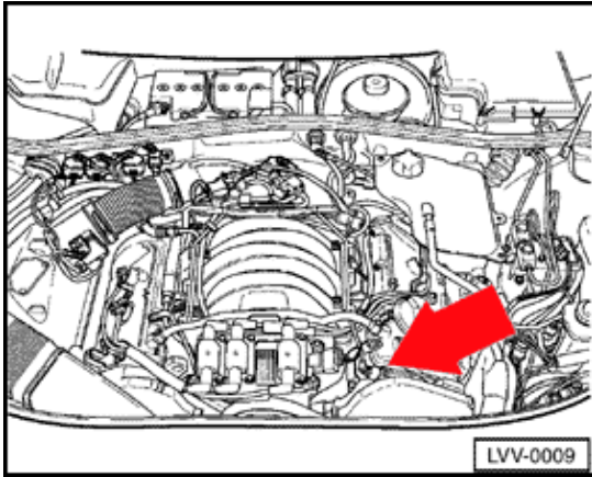
N208 Valve 2 for camshaft adjustment (2.8 ltr. engine)
