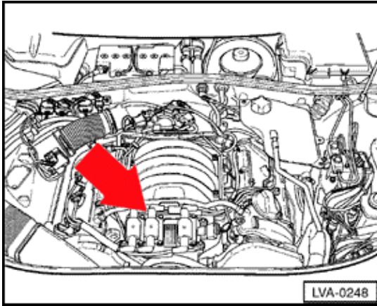
N158 Ignition coil 3 (2.8 ltr. engine)
