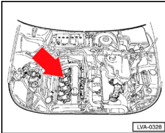
N158 Ignition coil 3 (1.8 ltr. engine)
