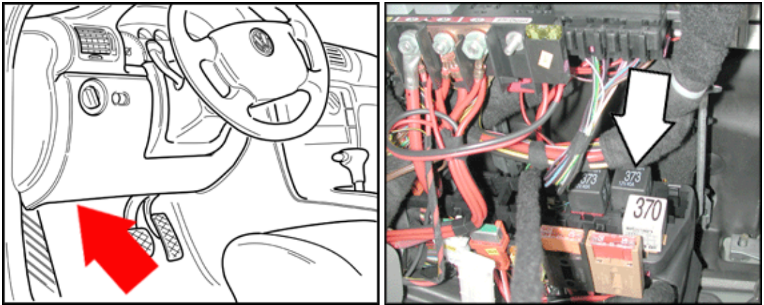
J397 Radiator Fan Afterrun Relay
