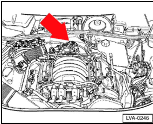
J338 Throttle valve control module (2.8 ltr. engine)
