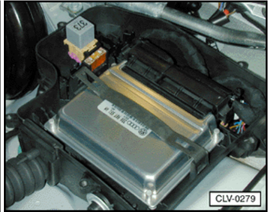
J220 Motronic Engine Control Module (ECM) (1.8 ltr. engine, from m.y. 2000)
