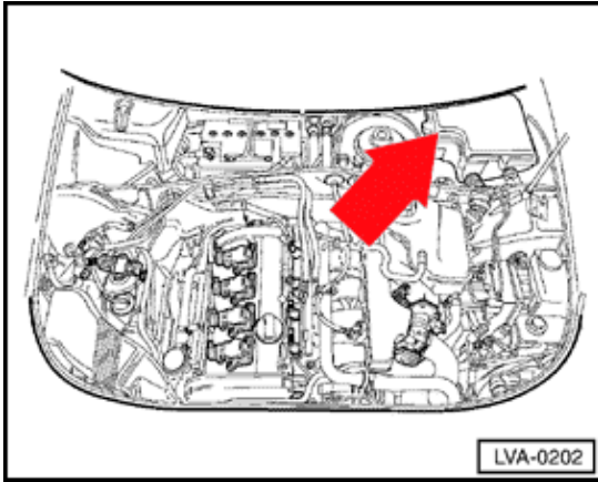
J220 Motronic Engine Control Module (ECM) (1.8 ltr. engine, from m.y. 2000)
