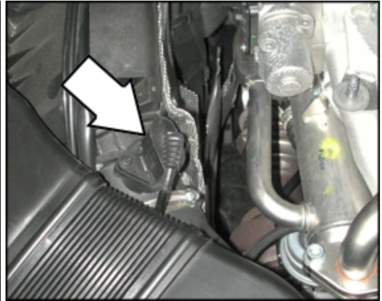
G70 Mass Air Flow (MAF) Sensor (2.0 ltr. tdi engine)
