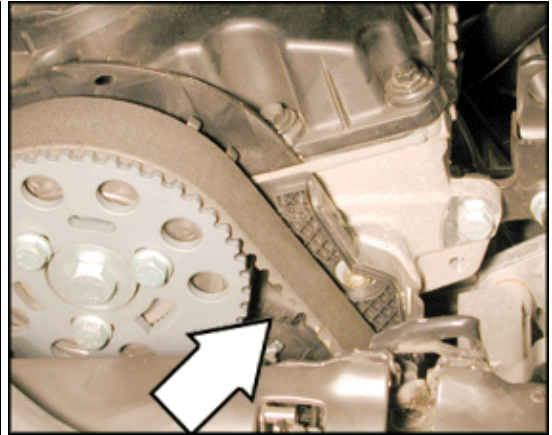
G40 Camshaft Position (CMP) Sensor (2.0 ltr. tdi engine)
