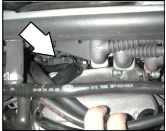
G300 Camshaft Position (CMP) Sensor 3 (4.0 ltr. engine)
