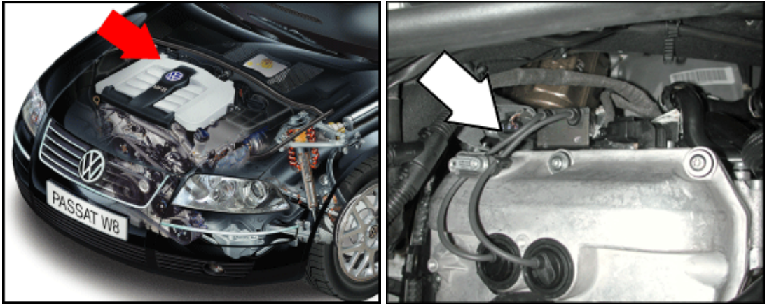
G163 Camshaft Position (CMP) Sensor 2 (4.0 ltr. engine)
