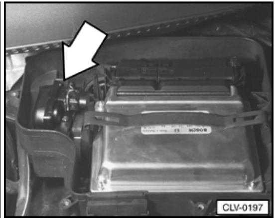
F96 Barometric Pressure (BARO) sensor (1.8 ltr. engine)
