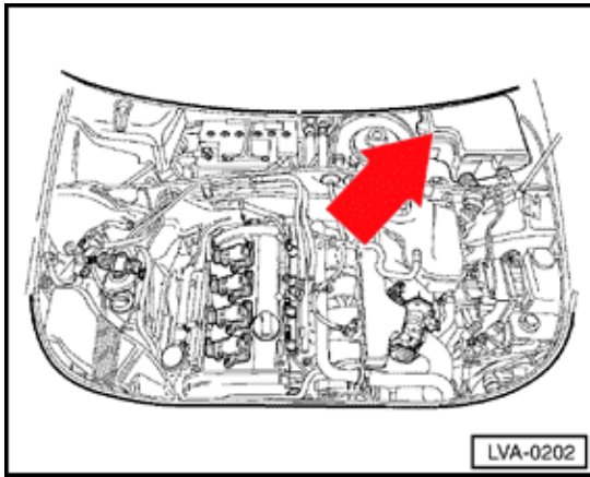
F96 Barometric Pressure (BARO) sensor (1.8 ltr. engine)
