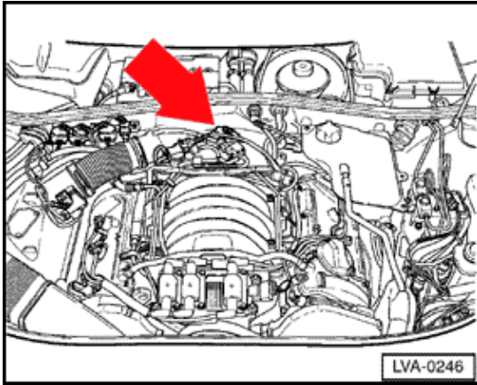
F60 Closed throttle position switch (2.8 ltr. engine)
