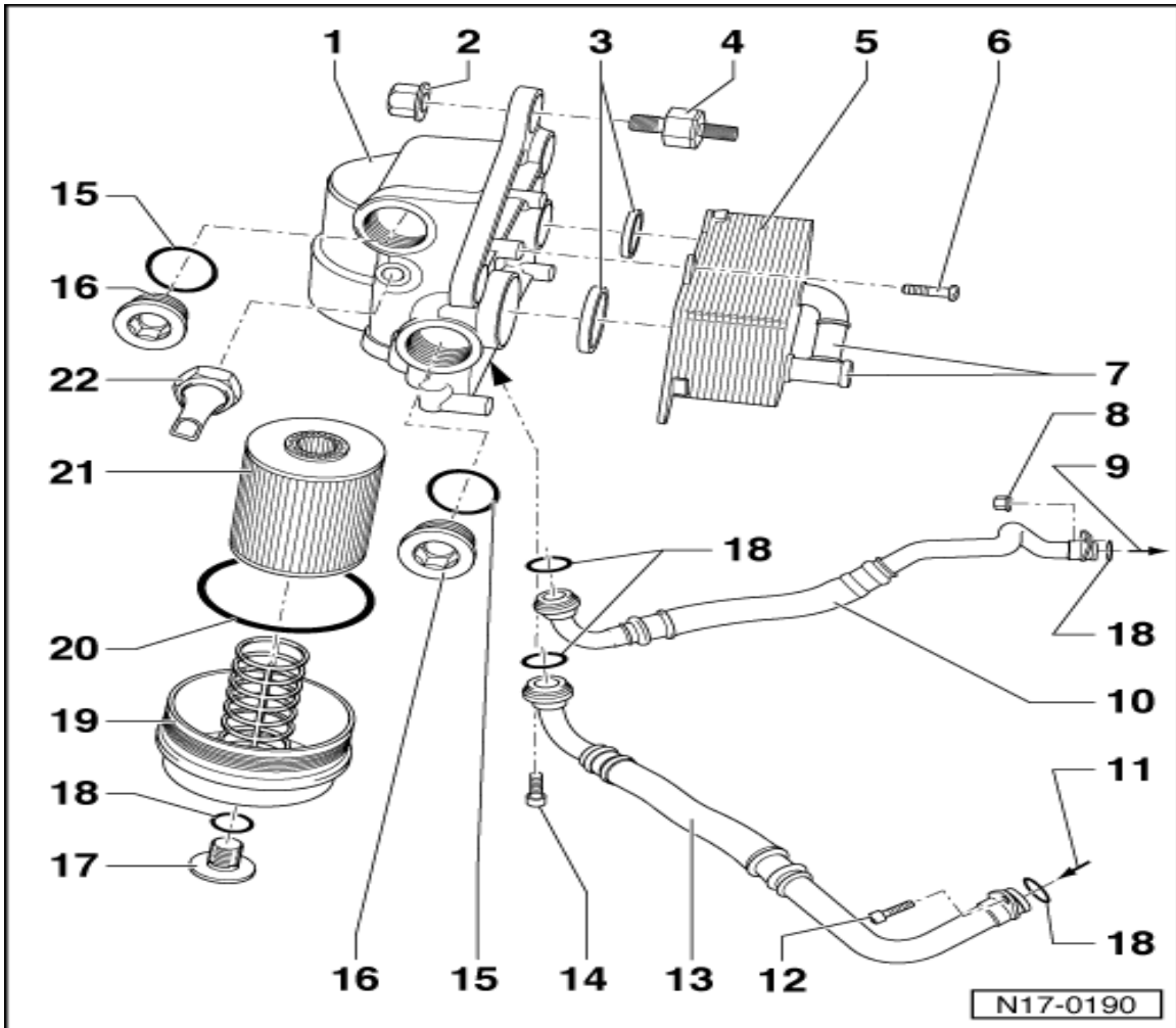
22 - Oil Pressure Switch -F1- at Oil filter adapter housing
